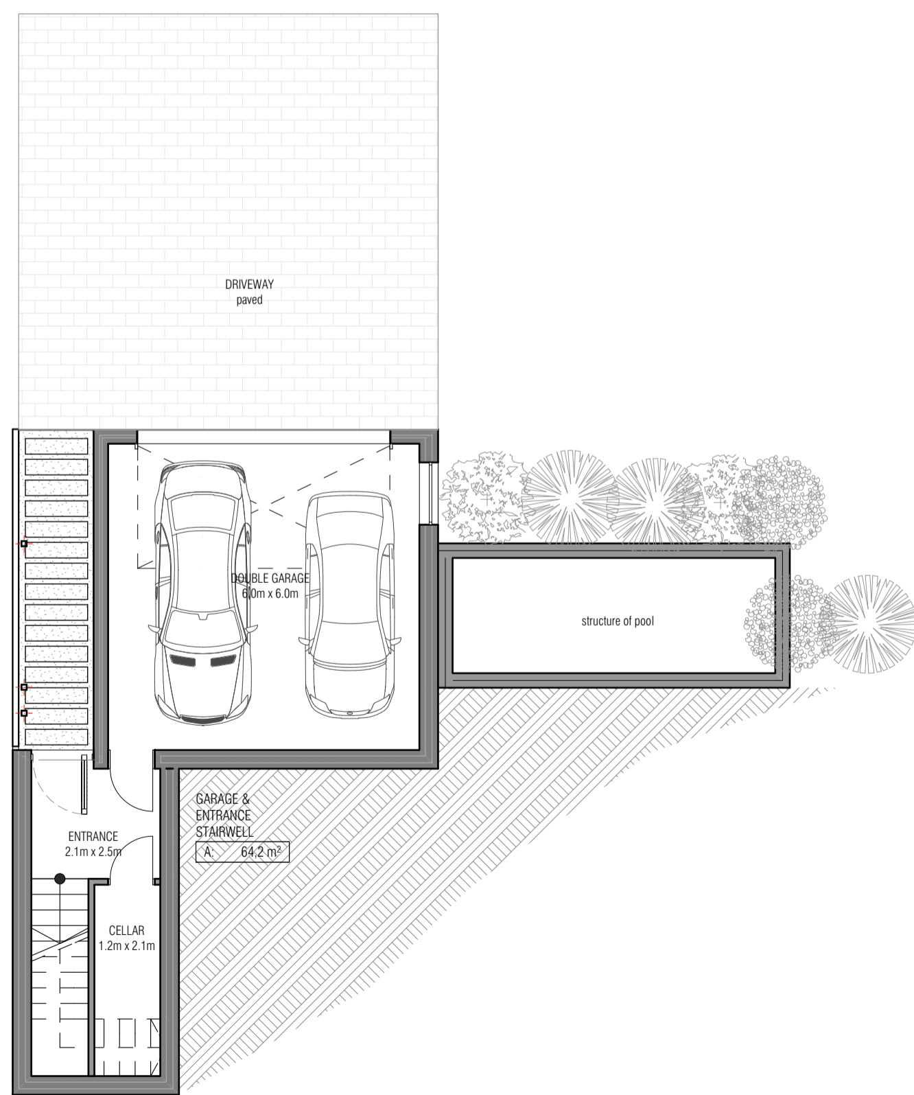
LOWER GROUND FLOOR PLAN 1:100
