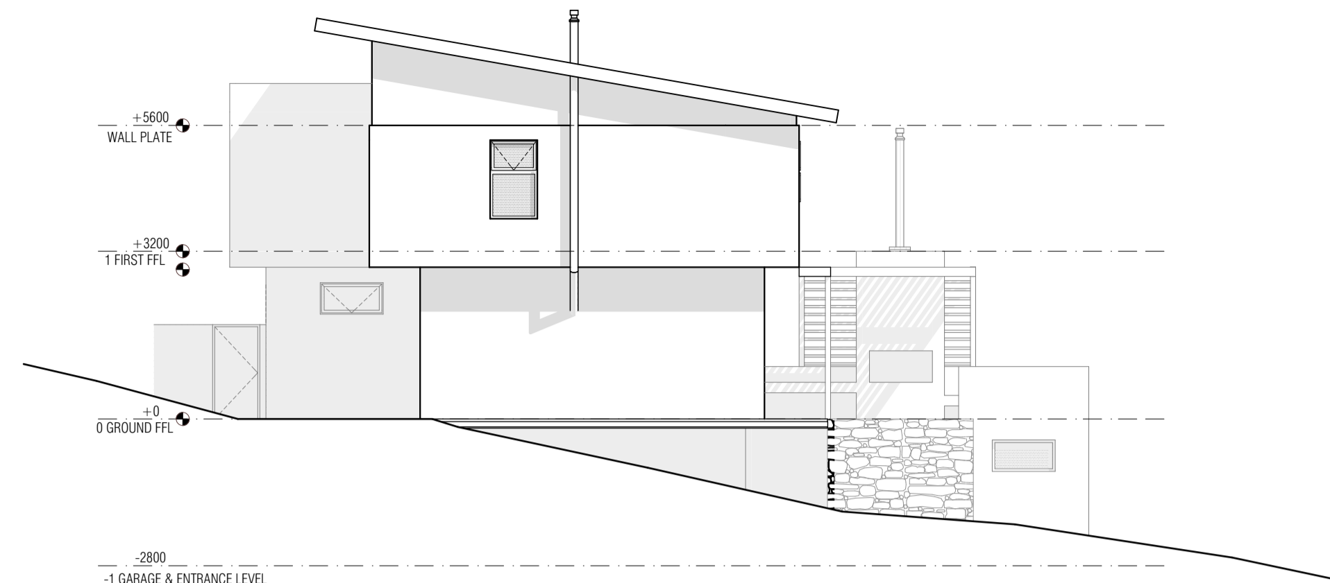
EAST ELEVATION 1:100
