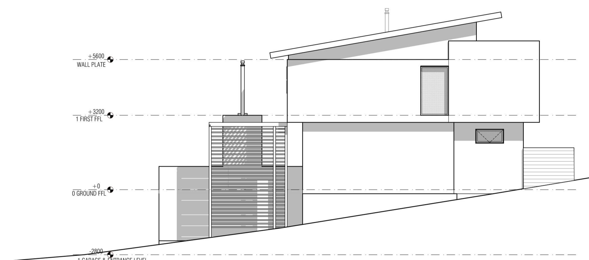
WEST ELEVATION 1:100
