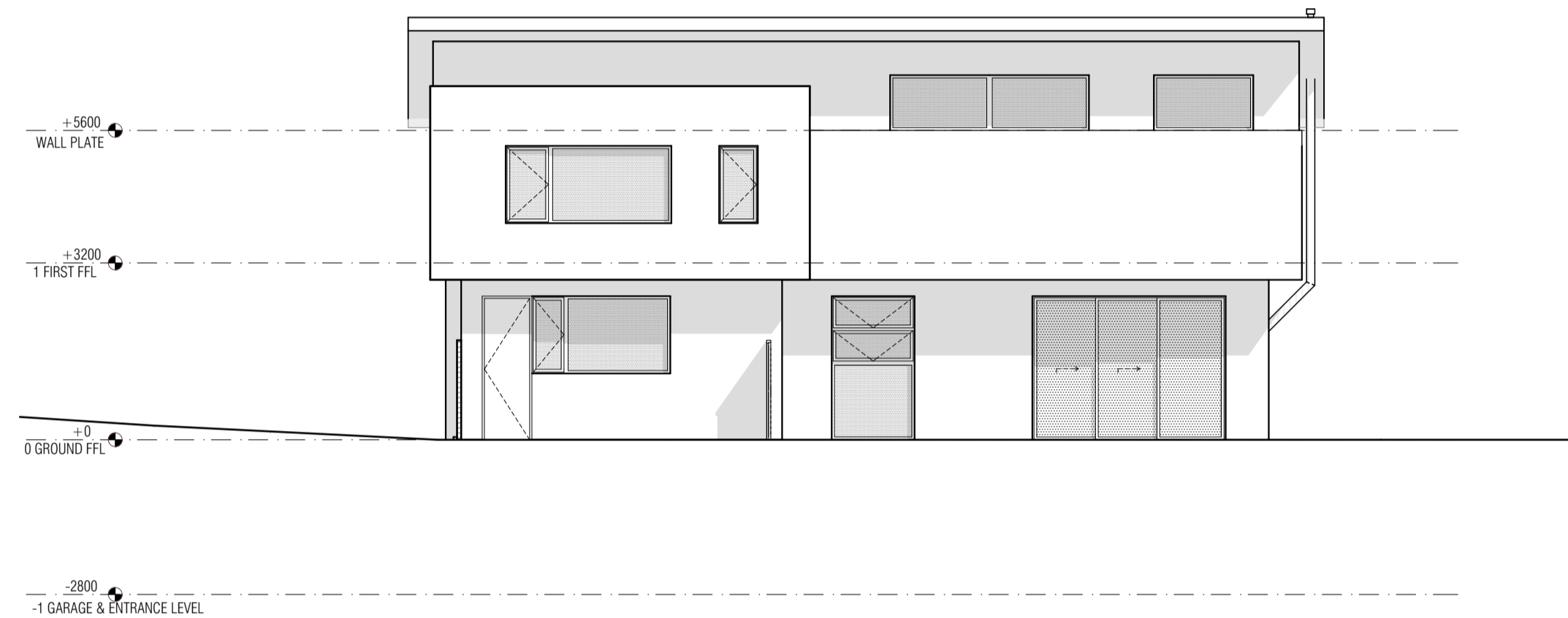
SOUTH ELEVATION 1:100
