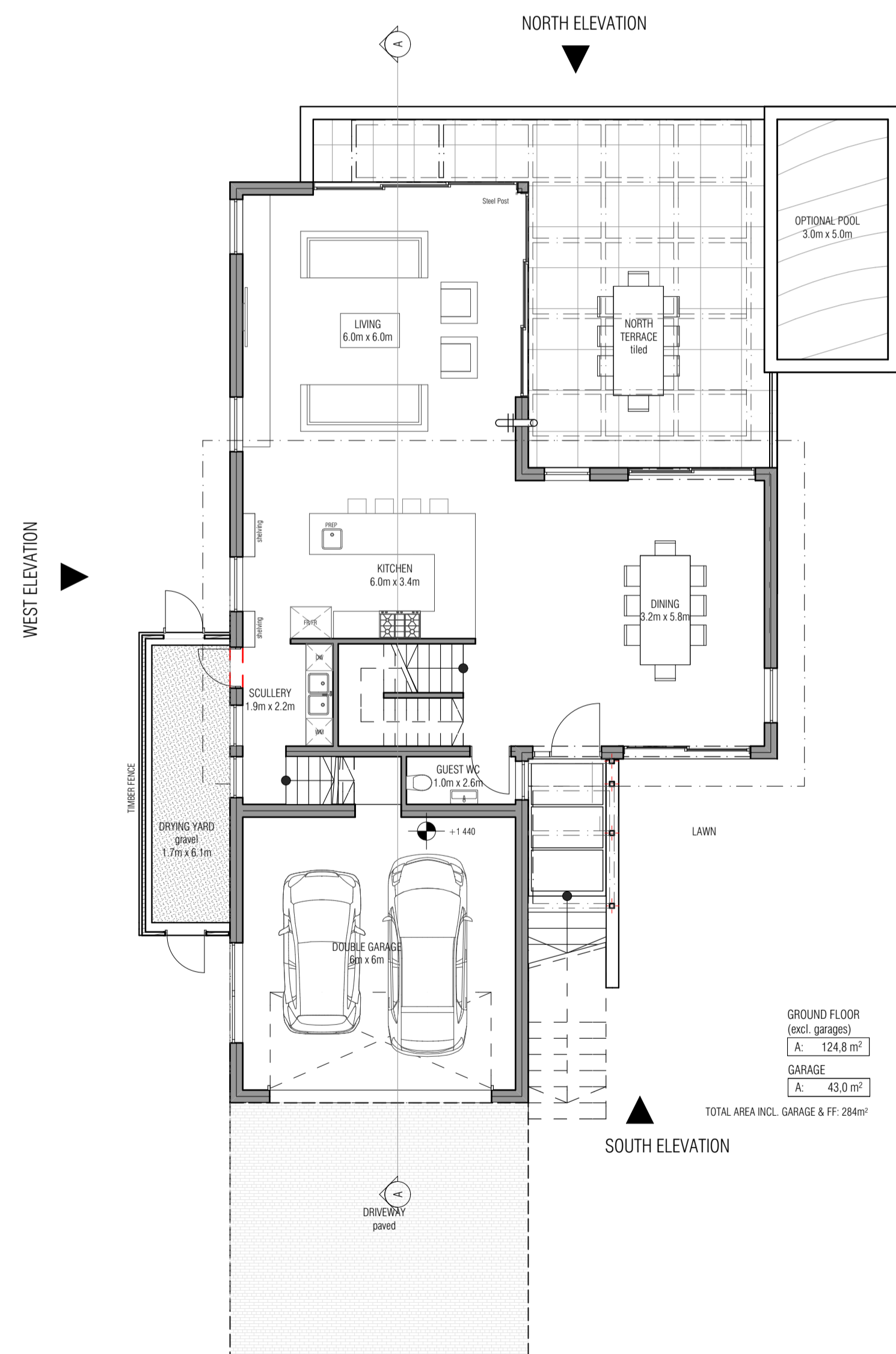
GROUND FLOOR 1:100
