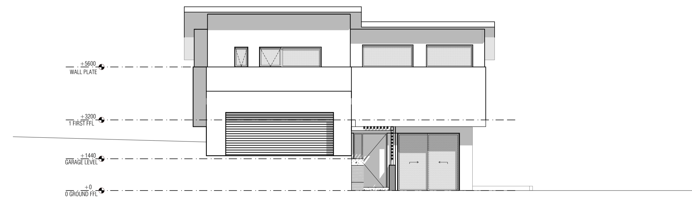
SOUTH ELEVATION 1:100
