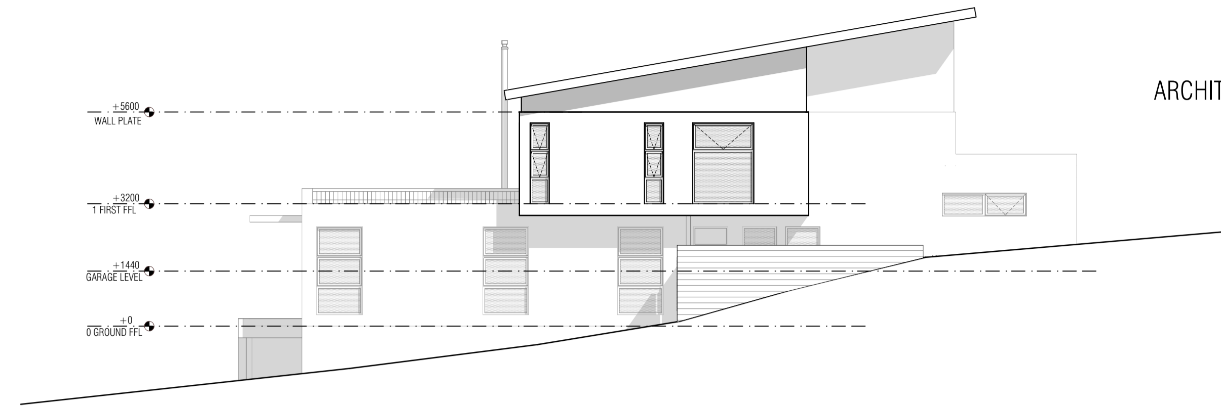
WEST ELEVATION 1:100
